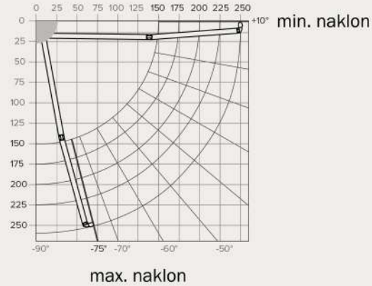
COMBI - DIM 250 DOUBLE-HOLE VERSION
