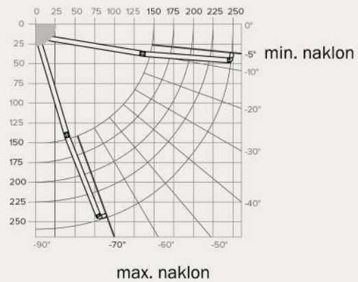
COMBI - DIM 250 SINGLE-HOLE VERSION
